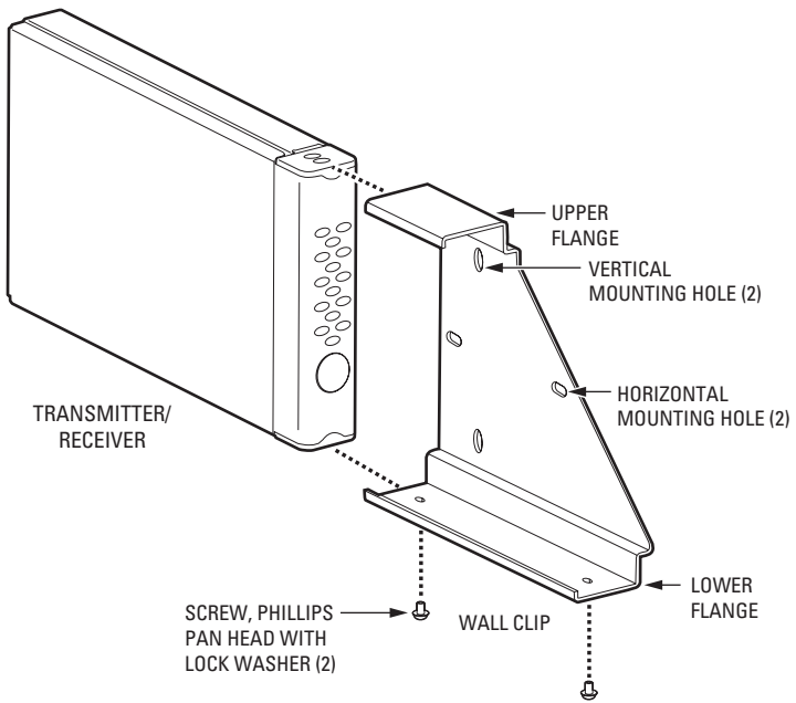
Figure 5. Mounting the FT85011 Transmitter/FR85011 Receiver Using the Wall Clip
